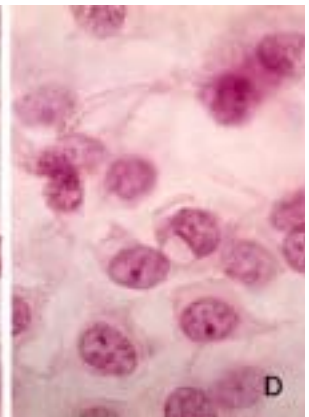
Fig. 2. Cytologic findings of chordoma. A. FNA smears show a myxoid fibrillary background. B. Strands and cords of physaliphorous cells and uniform smaller round cells are noted. C. Larger physaliphorous cells have abundant cytoplasm with multiple bubble-like cytoplasmic vacuoles. D. Smaller round to cuboidal cells are arranged in either cohesive clusters or scattered individually and have occasional vacuolization of the cytoplasm.
